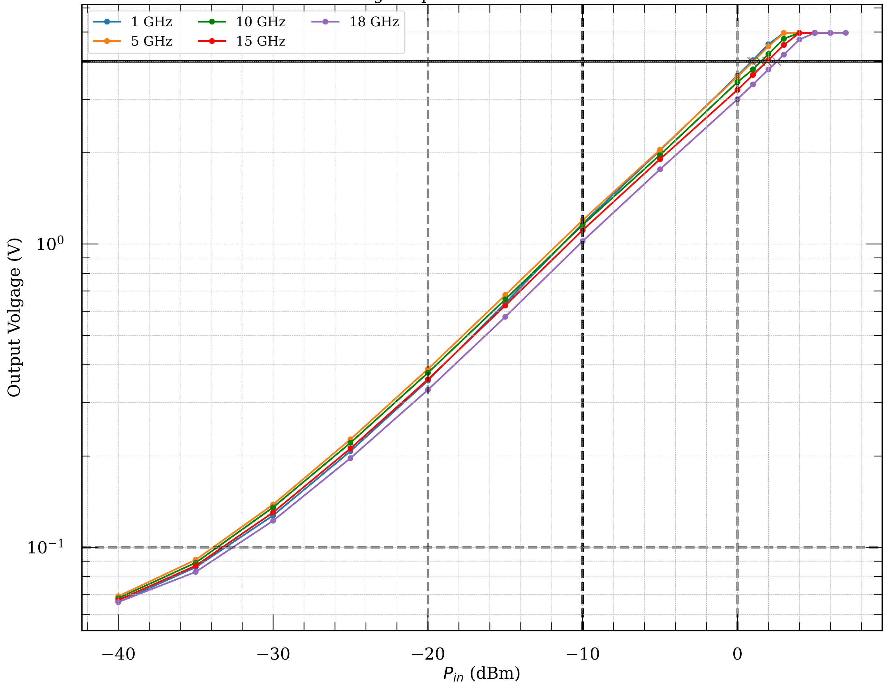
Measured voltage-to-power curve of detector module035
